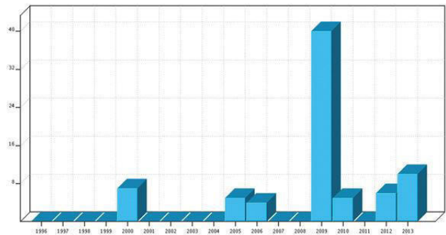
Figure 27: Trend of Human Life Loss by Storm (1996-2013)
