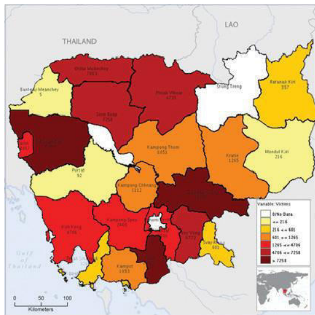
Figure 31: Thematic Map of Storm Victims (1996-2013)
