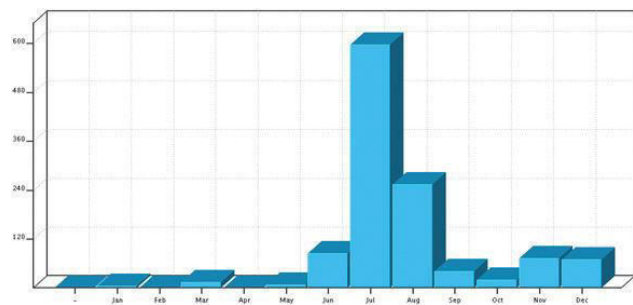
Figure 40: Seasonal Distribution of Drought Data Card (1996-2013)
