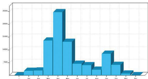
Figure 29: Seasonal Distribution of Storm Victims (1996-2013)
