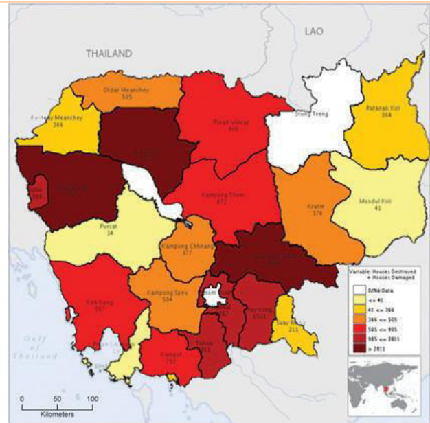
Figure 32: Thematic Map of Damaged and Destroyed Housing by Storm (1996-2013)
