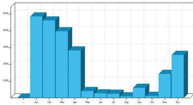
Figure 23: Seasonal Distribution of Fire Victims (2000-2013)
