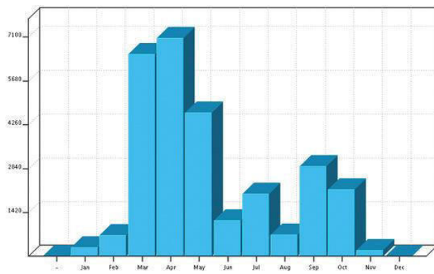
Figure 30: Seasonal Distribution of Damaged and Destroyed Houses by Storm (1996-2013)
